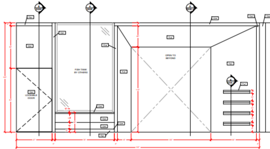
5 ELEVATION SCALE: 1/2"=1'-0" ARCH/RSF 11/18/24
